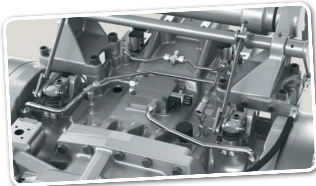
◀ ZF efficiency package – valve block from lubrication cut off.
